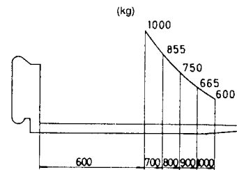
Load diagram
